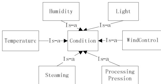
Fig. 4. The extended Condition ontology
