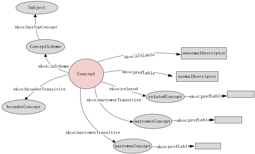
Fig. 2. SKOS Concept Model
