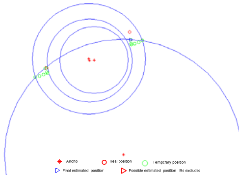
Fig. 5. The example of MSS algorithm process
