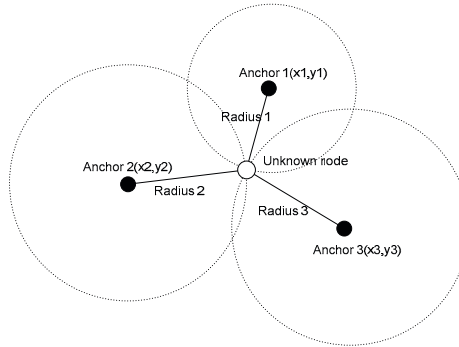
Fig. 1. Lateration localization scheme
