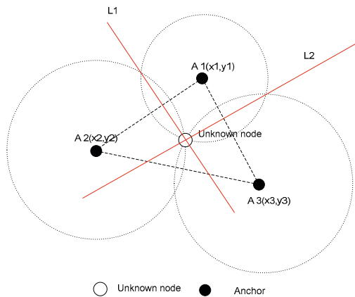
Fig. 3. The intesection of L1 and L2 is the estimated position
