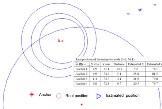
Fig. 4. Let different k th as the subtrahend, have different error
