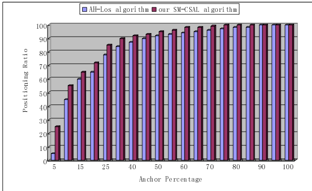
Fig. 10. Effect contrast between AH-Los and MSS-CSPL
