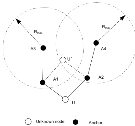
Fig. 6. Localization algorithm with only two 2-hop anchors
