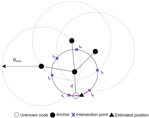
Fig. 7. The Localization algorithm with only one 1-hop anchor
