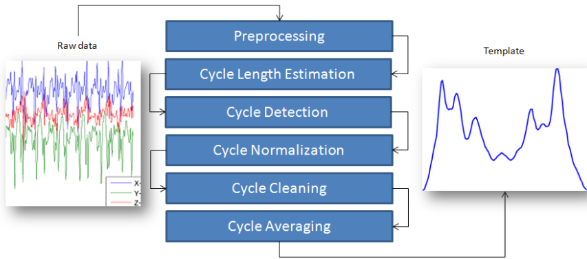
Fig. 1. Gait Analysis Overview
