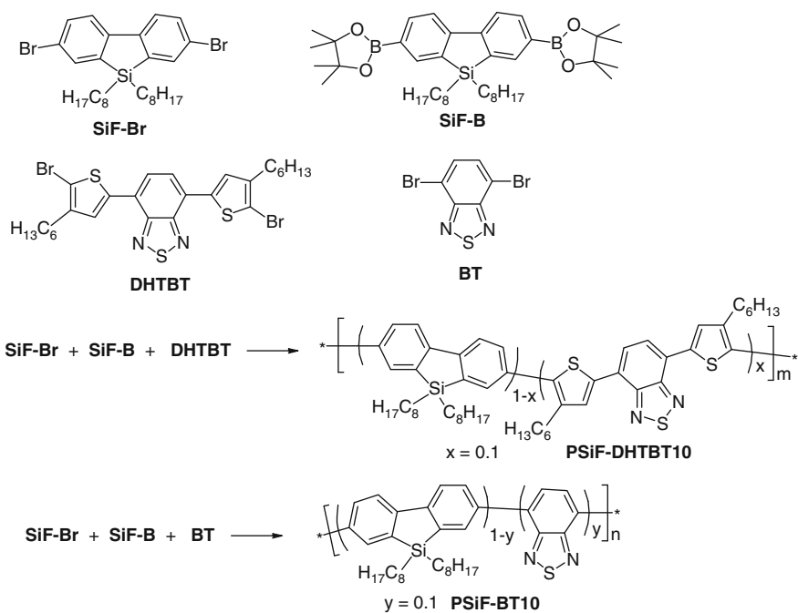
Scheme 20 Synthesis route of the polymer PSBTBT
