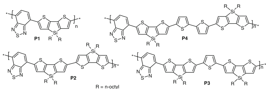
Fig. 48 Structures of PCPDTBT, PSiFDBT, and PSBTBT copolymers
