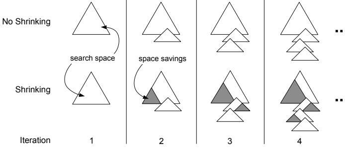
Fig. 1. Search Space Growth with and without Shrinking Technique. Dark regions represent shrunk search space (memory savings).
