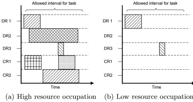
Fig. 3. Two different tasks and the current reservations on their available resources
