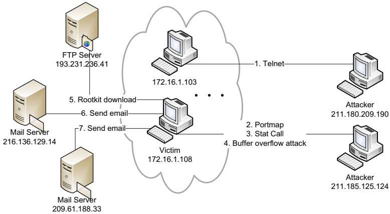
Fig. 3. Attack scenario
