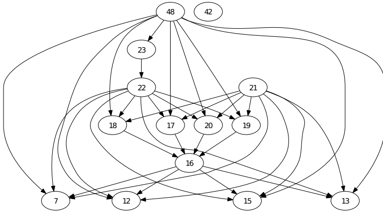
Fig. 4. NetFlow dependencies
