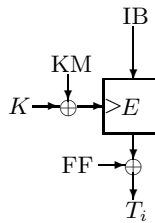
Fig. 1. In the keyed PGV model, a basic function f(K, M_i, T_{i-1}) is defined as f(K, M_i, T_{i-1}) = E(K \oplus KM, IB) \oplus FF , where K \xleftarrow{\$} \mathcal{K}_E and IB, KM, FF \in \{M_i, T_{i-1}, M_i \oplus T_{i-1}, \text{Cst}\}
