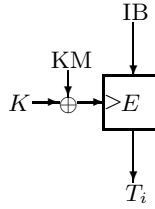
Fig. 3. In Compact PGV model with secret key K \xleftarrow{\$} \mathcal{K}_E , a block cipher E has two inputs: an input block IB and a key mask KM . A basic function g(K, M_i, T_{i-1}) is defined as g(K, M_i, T_{i-1}) = E(K \oplus KM, IB) , where IB, KM \in \{M_i, T_{i-1}, M_i \oplus T_{i-1}, Cst\} .
