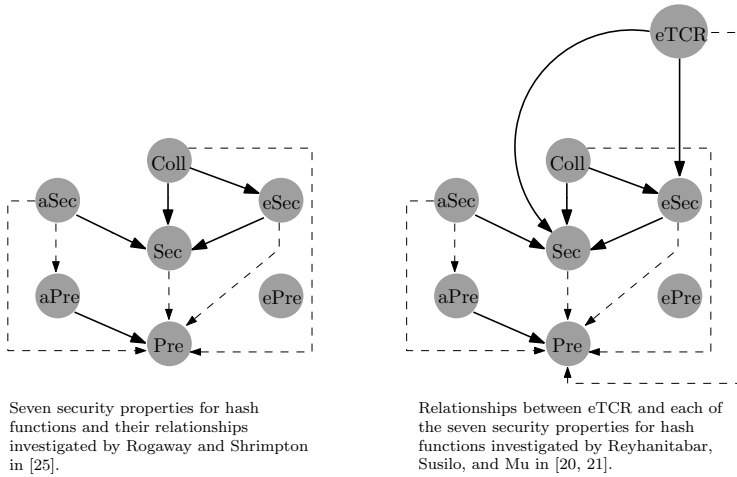
Fig. 1. Known relationships among the security notions for dedicated-key hash functions: a directed path shows an implication (dashed lines represent “provisional implications” in which the strength of the implications depends on the amount of compression achieved by the hash function) and lack of a path shows a separation [24, 25, 20, 21].
