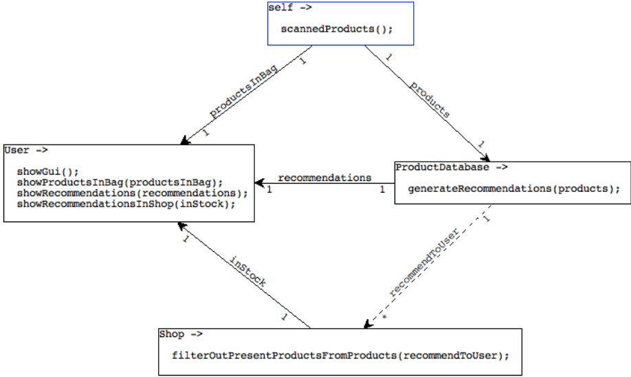
Fig. 2. AmbientTalk visual dataflow example
