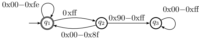
Fig. 1. DFA for B
