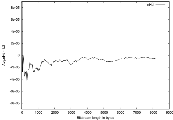
Fig. 2. Average \text{nHd}-1/2 of 10.000 random string pairs of B
