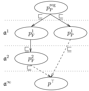
Fig. 1. A simple emergency attribute hierarchy
