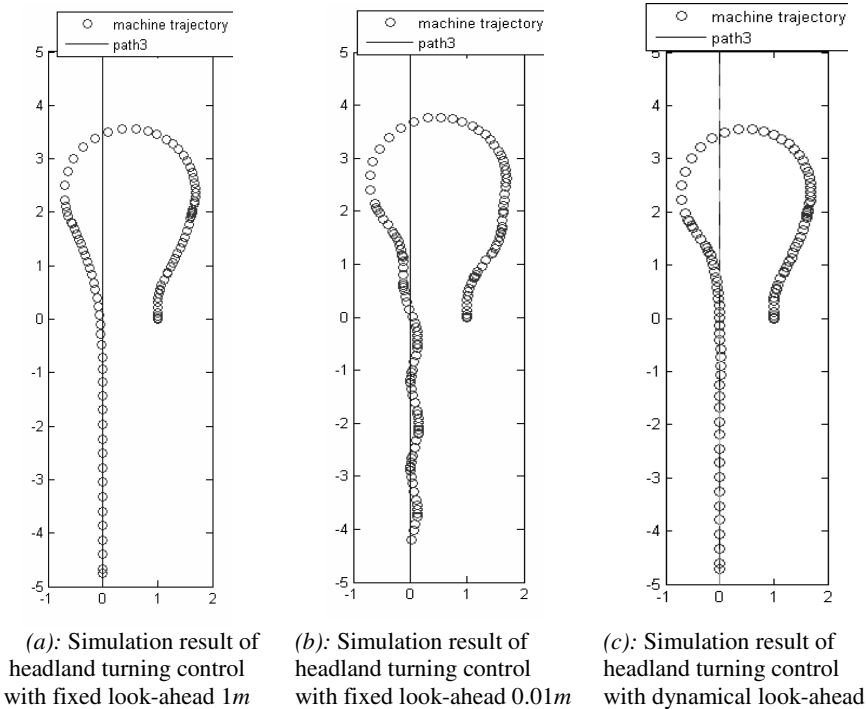
Fig. 4. Simulation result of headland turning control with different look-ahead distance
