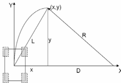
Fig. 1. Geometry of the Pure Pursuit Model
