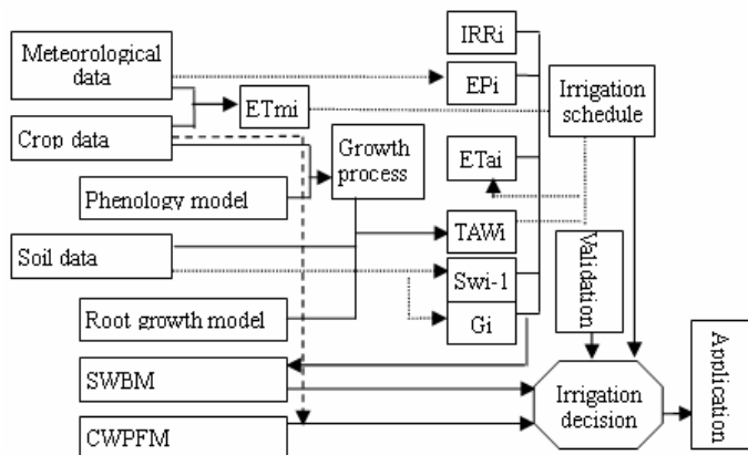
Fig. 1. Irrigation flowchart of CropIrri
