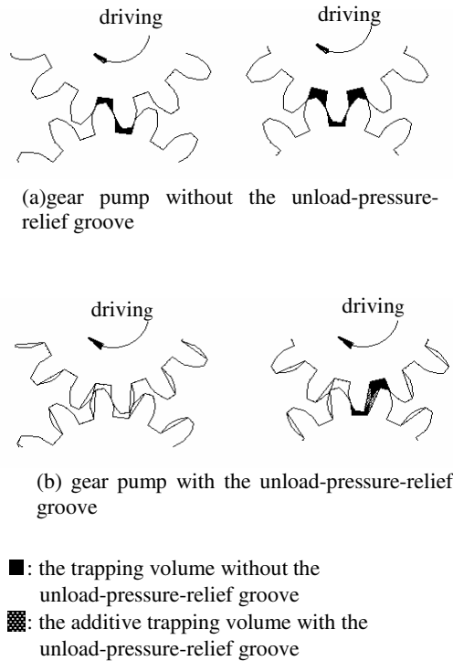
Fig. 3. Relation of gear pump without the unload-pressure-relief groove and with the unload-pressure-relief groove
