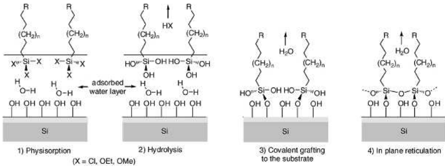
Fig. 2. Steps involved in the mechanism of SAM formation on a hydrated silicon surface [6]
