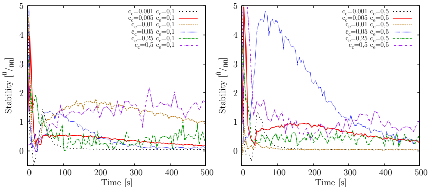
Fig. 2. Stability (Vivaldi NE CA, Azureus dataset)
