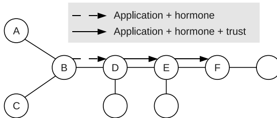
Fig. 1. Forwarder algorithm
