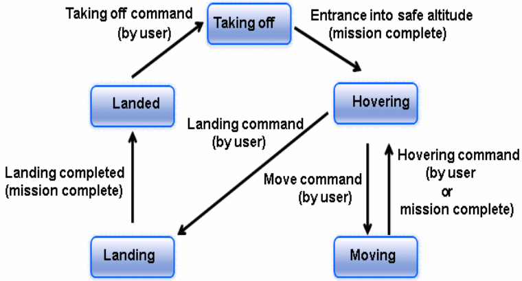
Fig. 3. Flight Mode Transition
