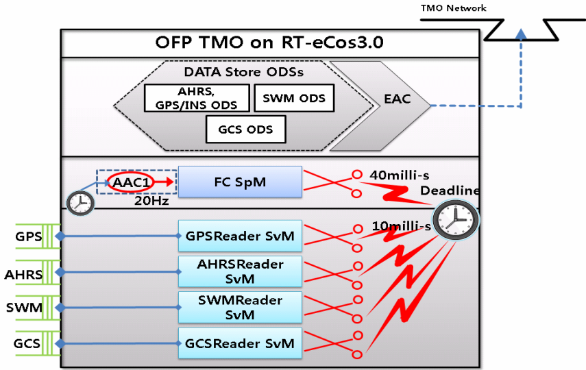
Fig. 4. Structure of the OFP-TMO
