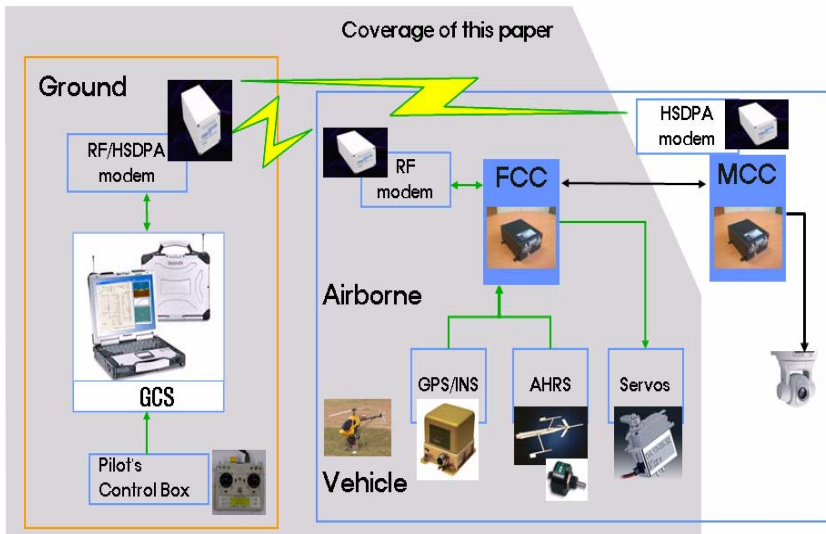
Fig. 2. Structure of the HELISCOPE
