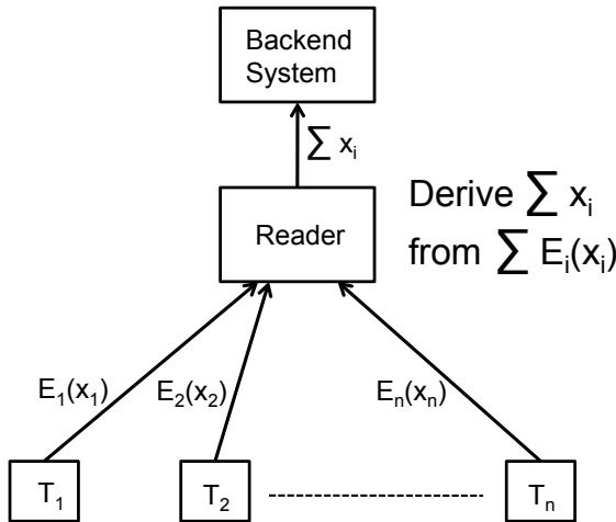
Fig. 1. Aggregation Protocol
