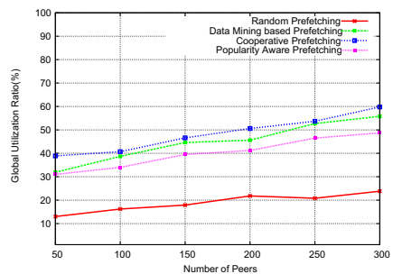
Fig. 4. Comparison of Utilization Ratio
