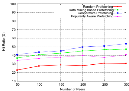
Fig. 3. Comparison of Hit Ratio
