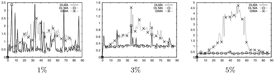
Fig. 9. Dissimilarity between M(R_\theta(X)) and R_\theta(M(X)) , for residual values 1%, 3%, 5%. Horizontal axis: \theta . Vertical axis: Dissimilarity.
