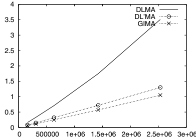
Fig. 10. Computing times (in seconds, vert. axis) versus image sizes (horiz. axis)
