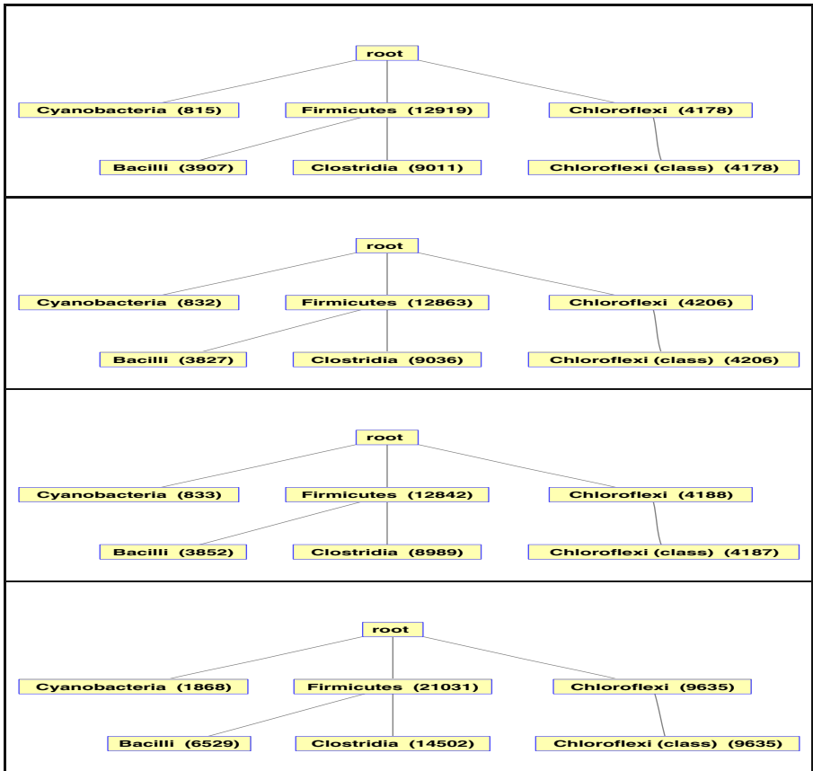
Fig. 1. Phylogenetic graph for M1. From top to bottom: LWproxy, GWproxy, EGWproxy and "Golden Truth".
