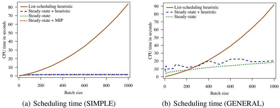
Fig. 5. Scheduling time in seconds
