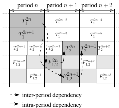
Fig. 2. A periodic schedule with inter-period and intra-period dependencies
