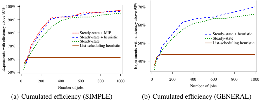
Fig. 4. Cumulated efficiency
