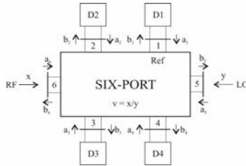
Fig. 1. Principle of the SPR [10]
