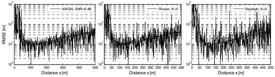
Fig. 8. RMSE [m] versus BN position for different channels
