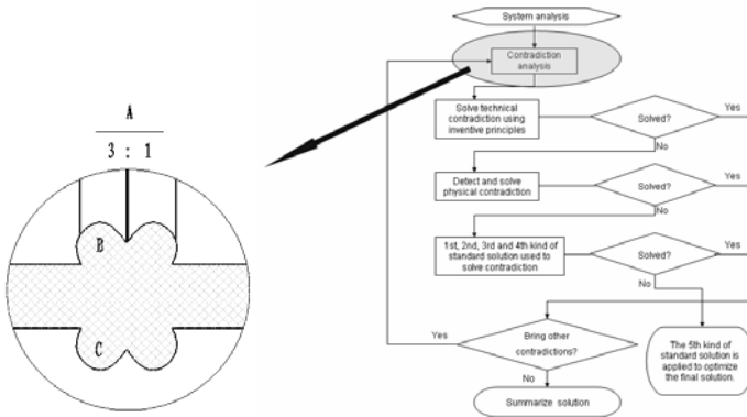
Fig. 5. Analysis of the first physical contradiction
