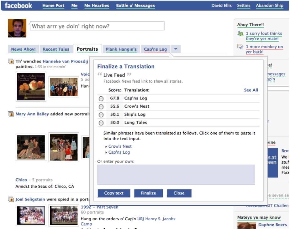
Fig. 2. Inline approval mode, in the English (Pirate) locale
