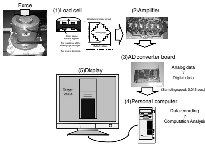
Fig. 2. Experimental setup
