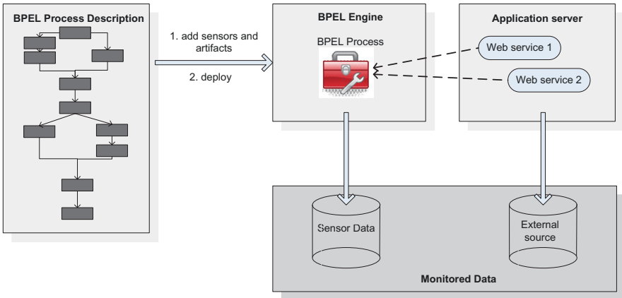
Fig. 2. The framework
