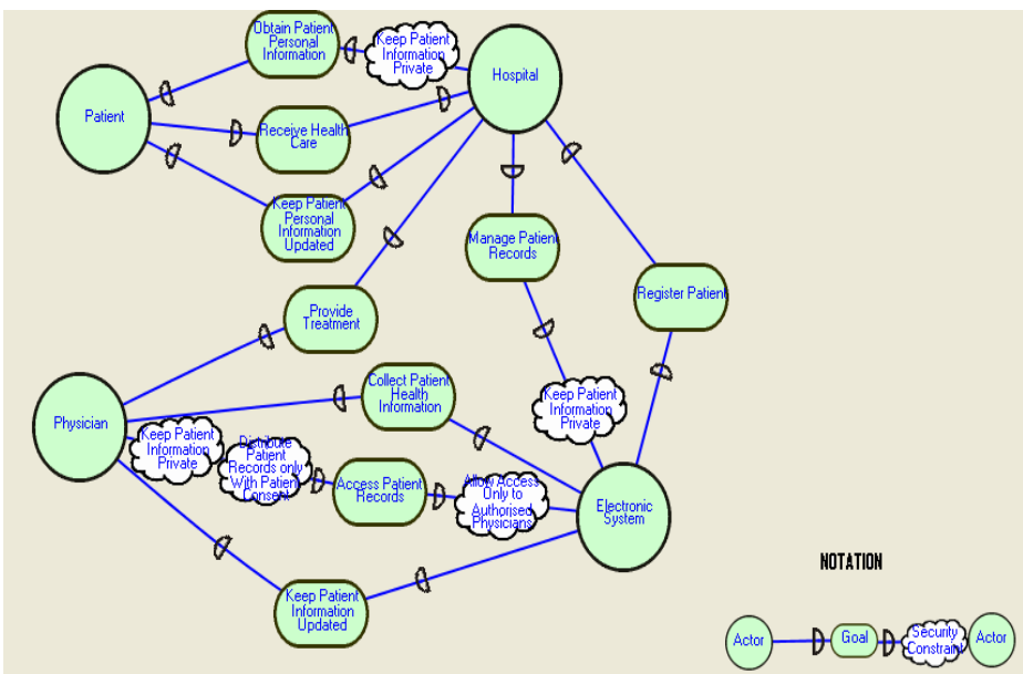
Fig. 1. secure Tropos security enhanced actor diagram
