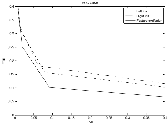
Fig. 3. ROC curves representing the matching performance of individuals based on the SIFT representation extracted from the left and right iris and the feature level fusion of the two irises
