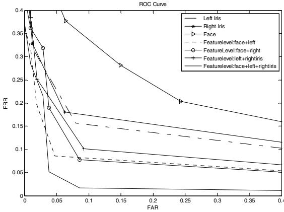
Fig. 4. ROC curves representing the matching performance of individuals based on the SIFT representation extracted from the face, the left and the right iris and the feature level fusion of the three traits
