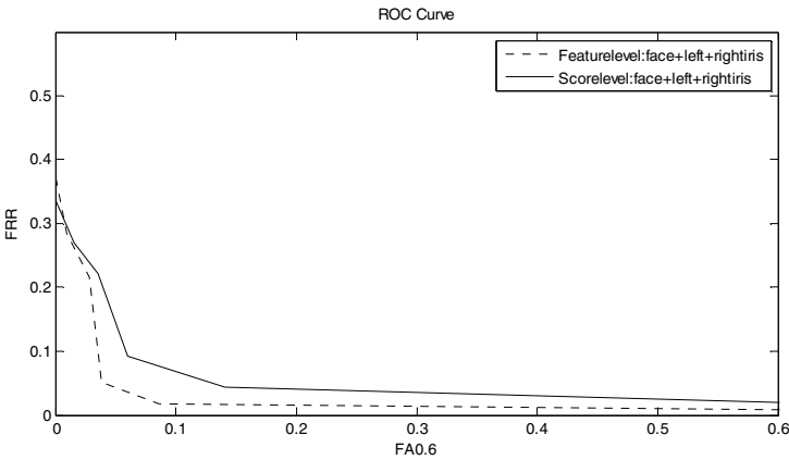
Fig. 5. Comparison of the feature level fusion, of the SIFT representations of the face, the left and the right irises, with the score level fusion of the matching scores of the individual modalities
