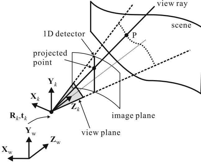
Fig. 3. Imaging geometry of a 1D camera. The world coordinate system is denoted by the \mathbf{X}_w , \mathbf{Y}_w and \mathbf{Z}_w axes. The camera coordinate system for the k -th camera is denoted by the \mathbf{X}_k , \mathbf{Y}_k and \mathbf{Z}_k axes. The relationship between the world and camera coordinate systems is given by the rotation matrix \mathbf{R}_k and translation vector \mathbf{t}_k . The world and camera coordinates of a 3D point P are \mathbf{p}_w = (x_w, y_w, z_w)^t and \mathbf{p}_k = (x_k, y_k, z_k)^t , respectively. The 1D detector (and hence the view plane) lies on the \mathbf{Y}_k - \mathbf{Z}_k plane.
