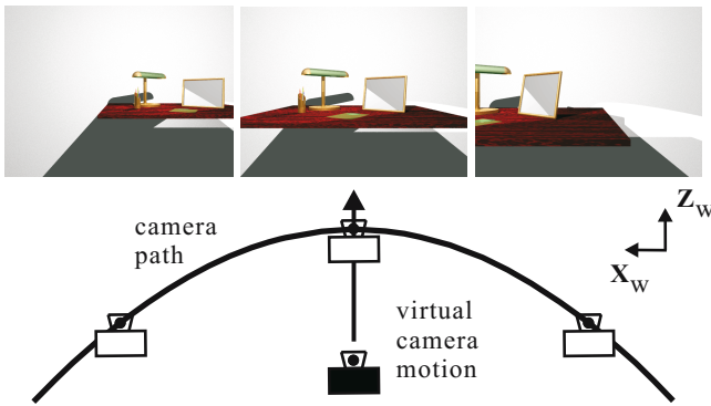
Fig. 5. The ray database obtained by POV-Ray [13]. The camera path was a sine curve. The virtual camera was the central one, as shown in Fig. 2 (a), and it was moved forward.
