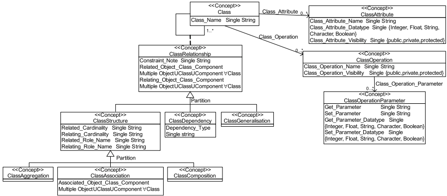
Fig. 2. Class diagrams ontology relations
