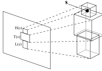
Fig. 1. The 3-box model of the human body: the state vector \mathbf{s} is transformed into the image space as the projection of a cuboid representing either the head, torso, or leg region. The projection of the cuboid is approximated by a rectilinear bounding box.
