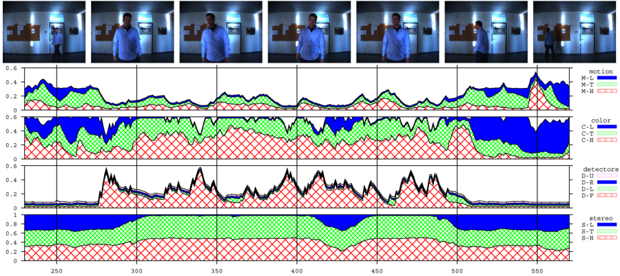
Fig. 4. Evolution of cue reliabilities in an example sequence. The three stereo cues constitute the first layer of the algorithm, their reliabilities sum up to 1. The remaining ten cues are used in layer 2 and sum up to 1 likewise. In the beginning of the interval, the subject approaches the camera. While he is walking (frame 250), the motion cues for legs and torso (M-L, M-T) contribute significantly to the track. At around frame 300, the subject's legs disappear, and in consequence the reliabilities of all leg-related cues (M-L, C-L, S-L) drop automatically. While the subject is standing in front of the camera (frames 300-500), the frontal face detection cue D-F and the the head color cue C-H dominate the track. The influence of the head color cue C-H drops dramatically, when the subject turns around (frame 520) and walks in front of the wooden pinboard, which has a skin-color like appearance.
