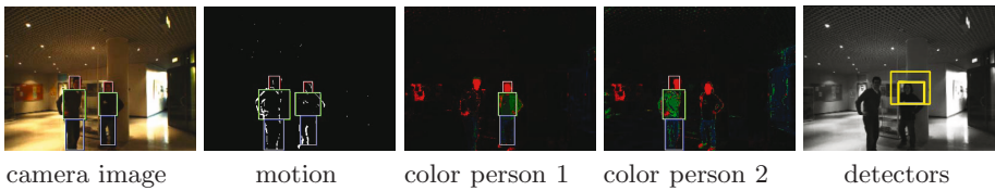
Fig. 2. Snapshot from a test sequence showing the different feature types. In this visualization, the color support maps for head, torso and legs of the respective person are merged into the RGB-channels of the image. The tracking result is superimposed.
