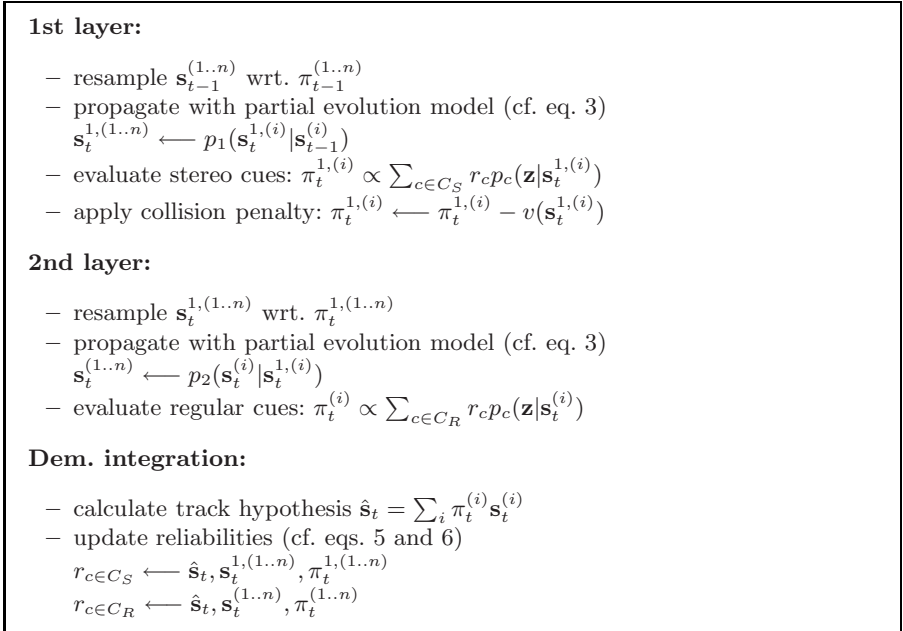
Fig. 3. Two-stage layered sampling algorithm with democratic cue integration
