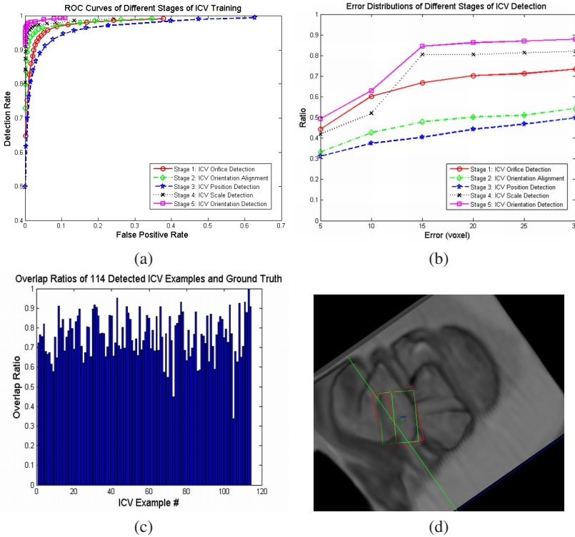
Fig. 5. (a) Receiver operating characteristic curves of different stages of training in our Ileo-Cecal Valve detection system. (b) Error ratio curves of top 100 ICV hypotheses of different stages of detection. Each curve show the ratios of hypotheses (Y axis) under the particular error readings (X-axis) against ground truth. All numbers are averaged over the testing sets of volumes, under five-fold cross-validation of 116 total labeled ICV examples. (c) Overlap ratios between 114 detected ICV examples and their ground truth. (d) A typical example of 3D ICV detection in CT Colonography, with overlap ratio of 79.8%. Its box-to-box distance as define in equation 8 is 3.43 voxels where the annotation box size is 29.0 \times 18.0 \times 12.0 voxels. Its orientational errors are 7.68^\circ , 7.77^\circ , 2.52^\circ with respect to three axes. The red box is the annotation; the green box is the detection. This picture is better visualized in color.
