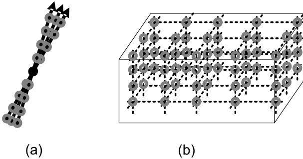
Fig. 3. Steerable sampling grid patterns for (a) 3D point detector and (b) 3D box detector
