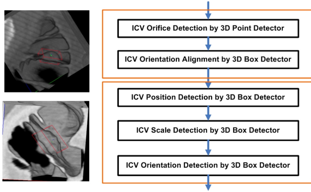
Fig. 2. System diagram of Ileo-Cecal Valve detection. The upper block is prior learning and the lower block is incremental parameter learning for ICV spatial parameter estimation. Examples of the annotated ICV bounding boxes are shown in red.
