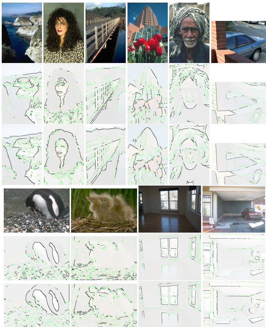
Fig. 6. Examples shown in three rows: input images, P_b , and multi- P_b (this work). Detected boundaries are discretized into two types: strong edge pixels (ranked 1-2000 in each image) in black, and weak edge pixels (ranked 2001-6000 in each image) in green. In such a way we visualize two points on the precision-recall curves in Figure 3 and 5. Large-scale boundaries are enhanced (i.e. from green to black, or from none to green), while small-scale boundaries, such as those found in texture, are suppressed (from black to green, from green to none).
