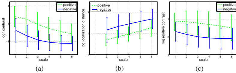
Fig. 2. Empirical distributions of boundary cues across scales. (a) Means and standard deviations of boundary contrast cues ( E ) at all 6 scales; in average, contrast is higher for positives or true boundaries. (b) Means and standard deviations of localization cues ( D ), distances to closest edge peaks; true boundaries are better localized. (c) Distributions of relative contrast ( R ); true boundaries are typically higher in contrast relative to its neighbors. We find all the cues informative. However, they are also noisy as shown by the large standard deviations.
