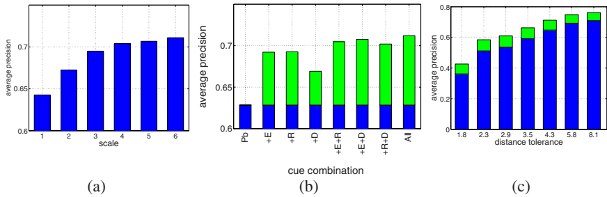
Fig. 4. Cue combination evaluated with average precision: (a) improvements in performance as we gradually add the number of scales; (b) improvements over default scale Pb by adding subsets of features, including contrast (E), localization (D), and relative contrast (R); (c) improvements over Pb with different choices of distance tolerance in evaluation
