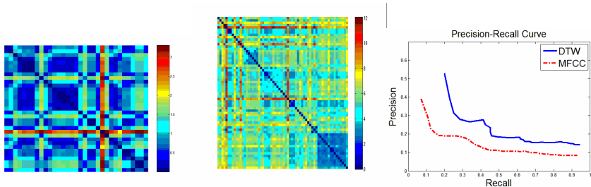
Fig. 8. Illustration of the comparison between shape-based time warping and MFCC algorithm for pair-wise discrimination. (a) Confusion matrix using our algorithm (b) Confusion matrix using MFCC.
