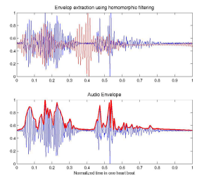
Fig. 5. Illustration of envelope curve extraction of sounds. (a) Homomorphic filtering-based low frequency approximation (shown in red), (b) perceptual envelope.
