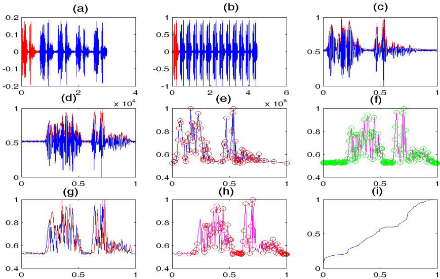
Fig. 7. Illustration of shape-based dynamic time warping
