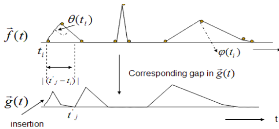
Fig. 6. Illustration of the shape matching problem for envelope curves
