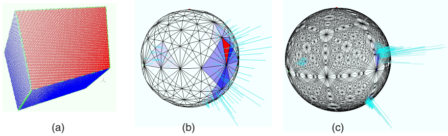
Fig. 3. A synthetic 3D image of a box (a) and its unified discrete Gaussian images for k = 1 (b) and k = 2 (c). Concerning cell colors on the discrete Gaussian sphere (b,c), the darker the blue cell, the larger the value of u(c) , and the red cell has the maximum value. The length of the pale blue needle for each cell c also corresponds to the value of u(c) . On a digitized box (a), red and blue points have linear LGPs for k = 1 , while green points have non-linear LGPs. Note that red points correspond to the red cell.
