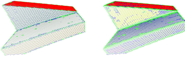
Fig. 4. A result of planar surface detection from a 3D range image of blocks for k = 1 (left) and k = 2 (right) with s = 100 . Four (resp. five) planar surfaces are detected for k = 1 (resp. k = 2 ) so that each surface is colored with a different color except for light green and blue. Light green points have non-linear LGPs and blue points have linear LGPs but cannot constitute a planar surface whose size is not less than s .
