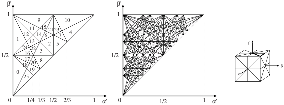
Fig. 2. Normal cells in the parameter space (\alpha', \beta') for k = 1 (left), k = 2 (center), and a cubical Gaussian sphere (right)
