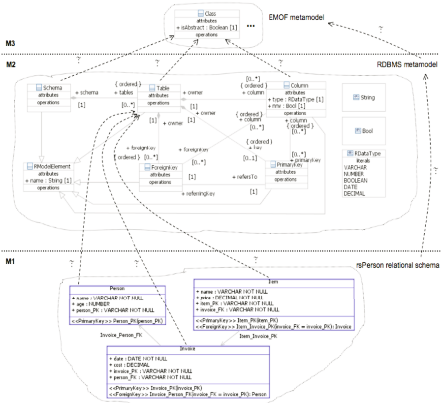
Fig. 2. The MOF framework
