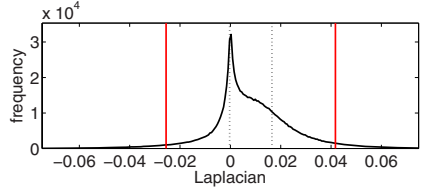
Fig. 5. Example Laplacian histogram for a fixed ADC range. Dotted lines indicate the lower and upper quartiles, solid (red) lines indicate the thresholds l_{min} and l_{max} respectively.
