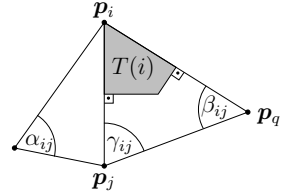
Fig. 4. Illustration of the weight computation for the discretization of the Laplace-Beltrami operator on a triangulated mesh
