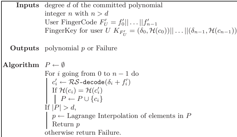
Fig. 2. Decoding algorithm: Secure sketch for a user pretending to be U
