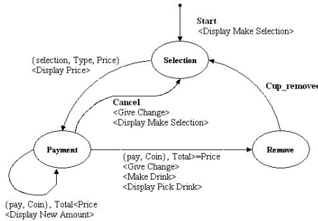
Fig. 9. FSM - coffee machine
