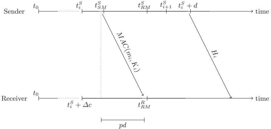
Fig. 5. Common Pattern for Delayed Key Disclosure Protocols
