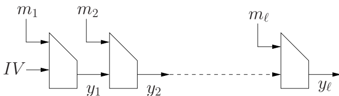
Fig. 1. The plain Merkle-Damgård Mode
