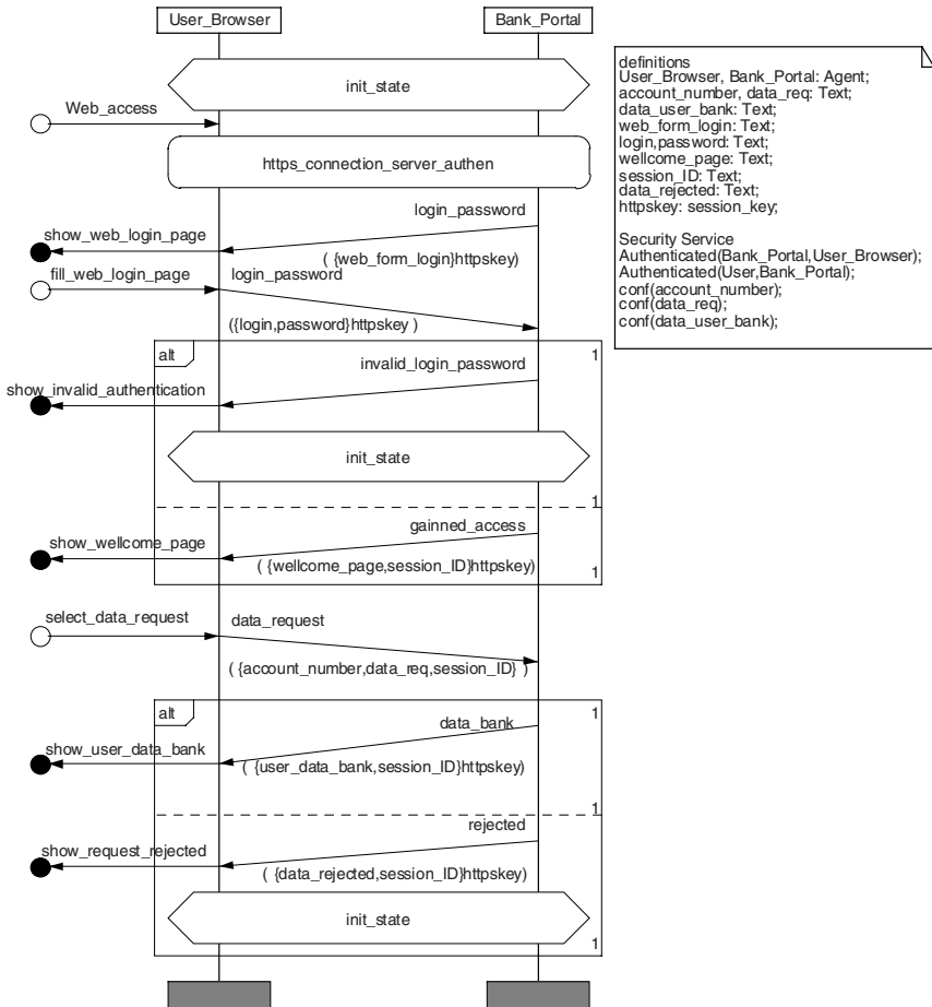
Fig. 3. SRSL security scenario of user’s access to data bank
