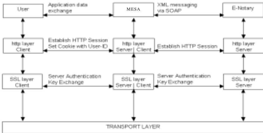
Fig. 5. Application structure in SRSL module description
