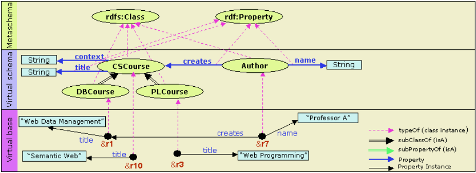
Fig. 3. A more complex RVL view
