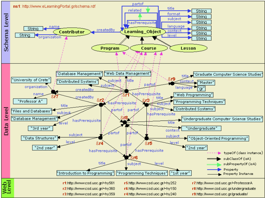
Fig. 1. An example e-Learning Portal application
