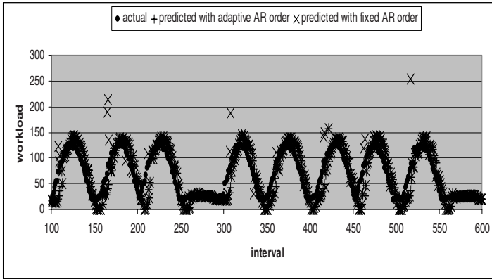
Fig. 2. Short term forecaster showing the comparison between an actual time series and 1 min (6 interval) ahead predicted values. Note that spurious predictions (e.g. high flyers) occasionally resulting from the fixed order model are greatly minimized with the adaptive order model
