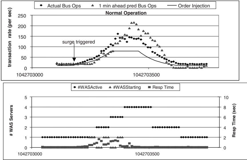
Fig. 6. Operation of system using dynamic surge protection
