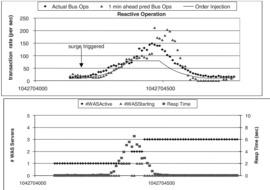
Fig. 7. Operation of system using a threshold-based heuristic
