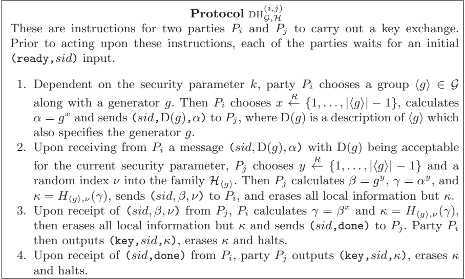
Fig. 4. Protocol \text{DH}_{\mathcal{G}, \mathcal{H}}^{(i,j)}
