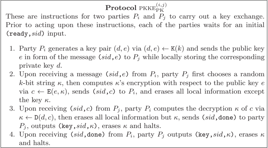
Fig. 5. Protocol \text{PKKE}_{\text{PK}}^{(i,j)}
