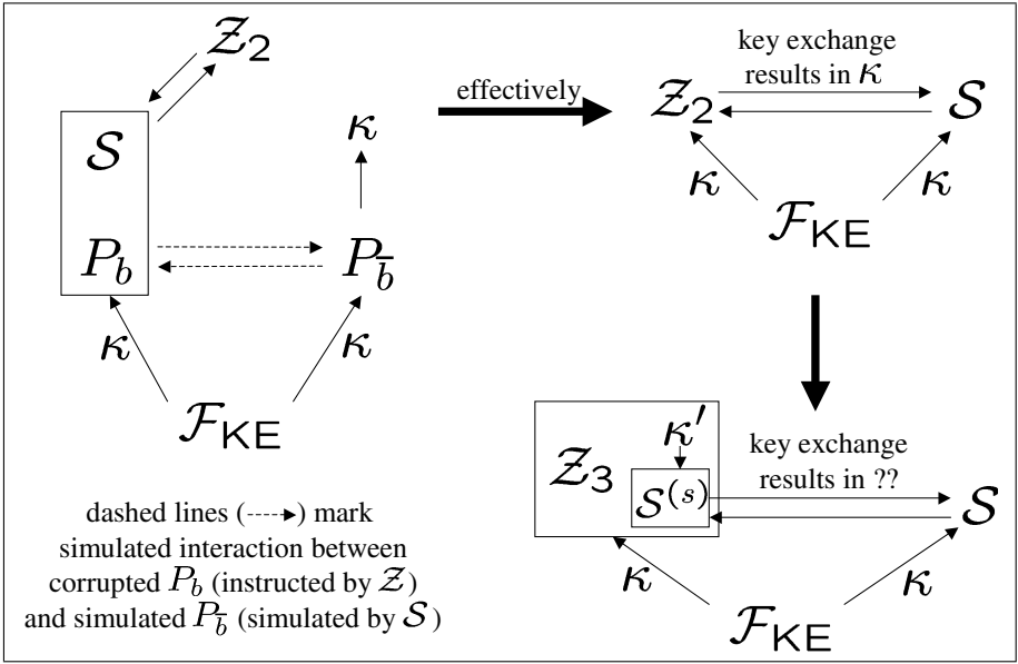
Fig. 2. The environments \mathcal{Z}_2 and \mathcal{Z}_3 from the proof of Proposition 1 in the ideal model
