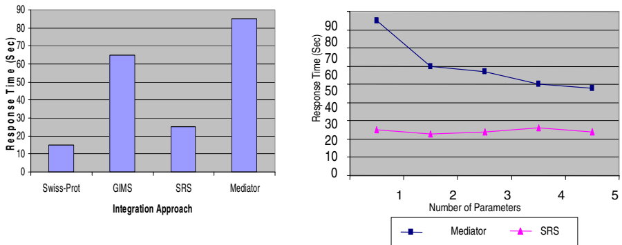
Fig. 2. Response Time for Querying Organism “Human Coronavirus” from Swiss-Prot for various integration methods; Comparison of Response Time for mediator and SRS for searching with various no of parameters
